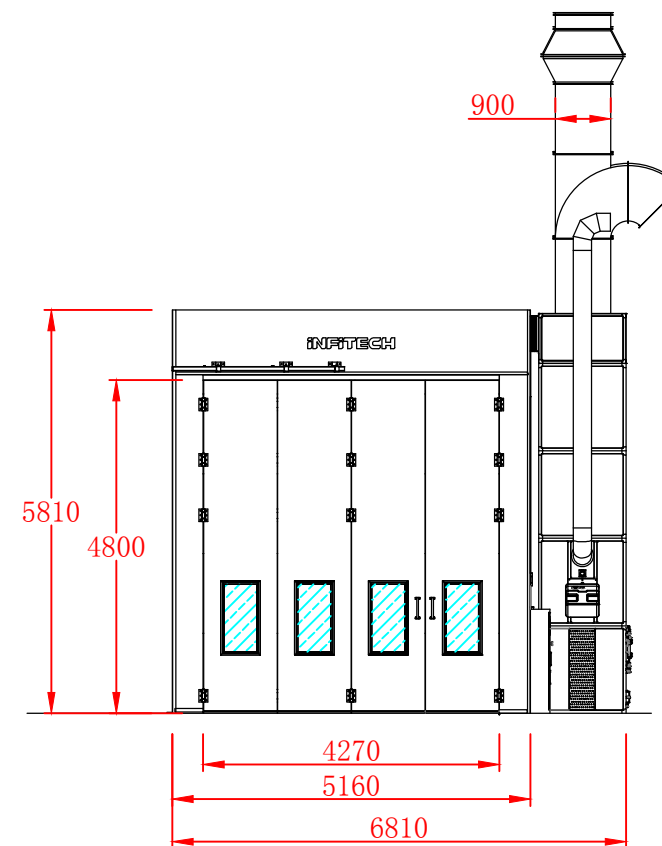
FRONTAL VIEW
