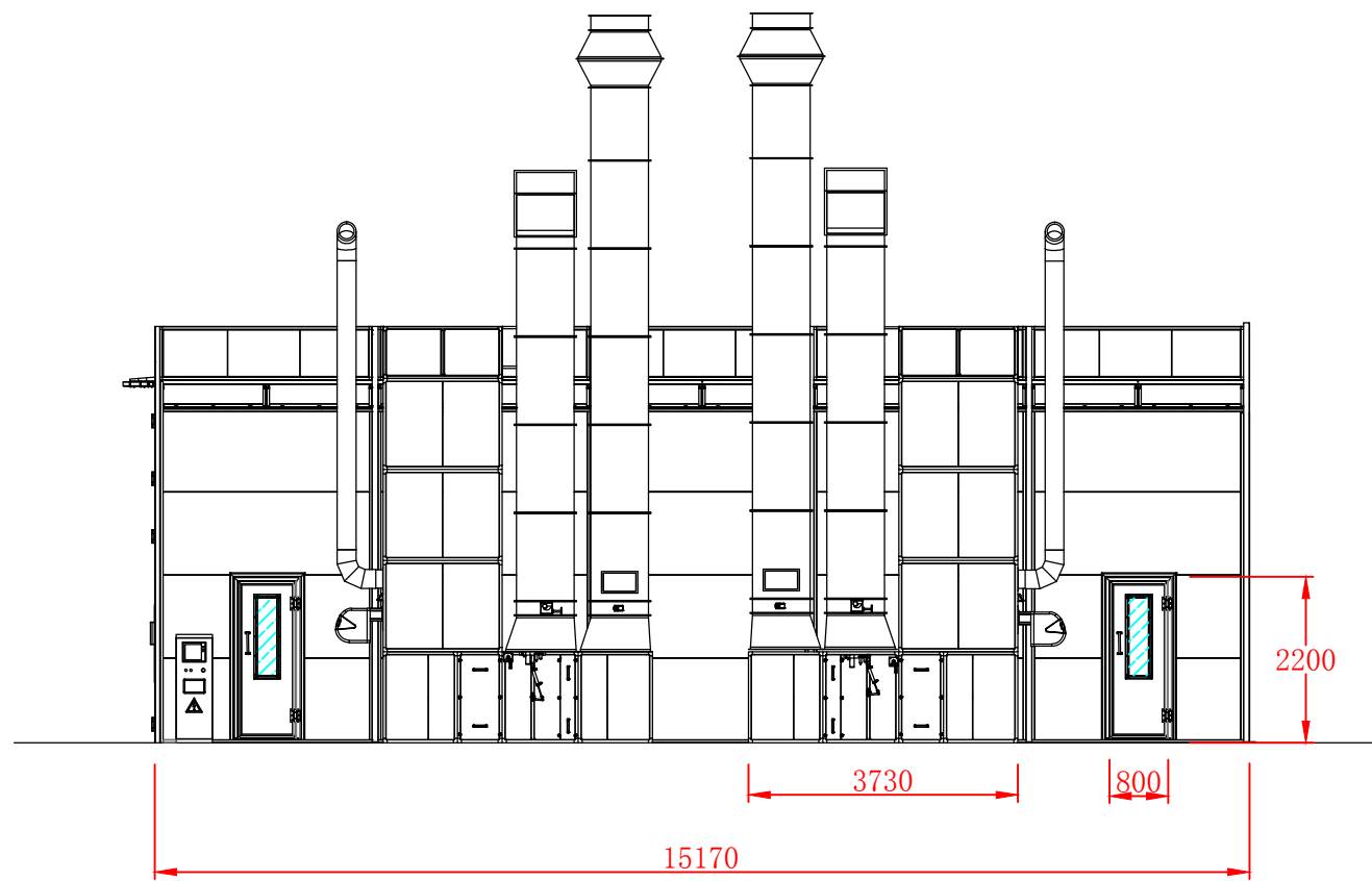
SIDE VIEW
