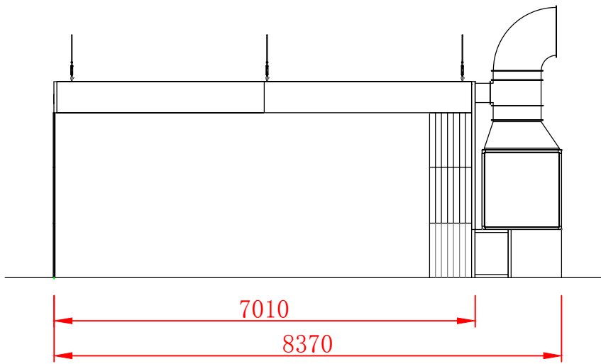
FRONTAL VIEW
